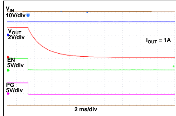
FIGURE 2-29: Enable Turn-Off.
