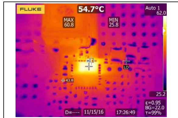
FIGURE 2-45: Thermal Picture ( I_{OUT} = 5A ).
