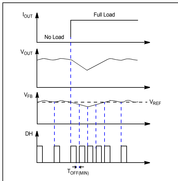
FIGURE 4-2: MIC28514 Load Transient Response.
