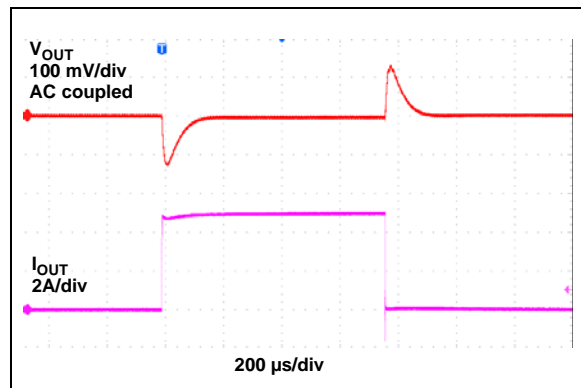
FIGURE 2-41: Load Transient Response (0 to 5A).
