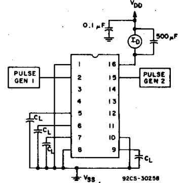
Fig. 11 — Dynamic power dissipation test circuit. NOTE: P.G.1 = f_{CL} ; P.G.2 = \frac{f_{CL}}{4}
