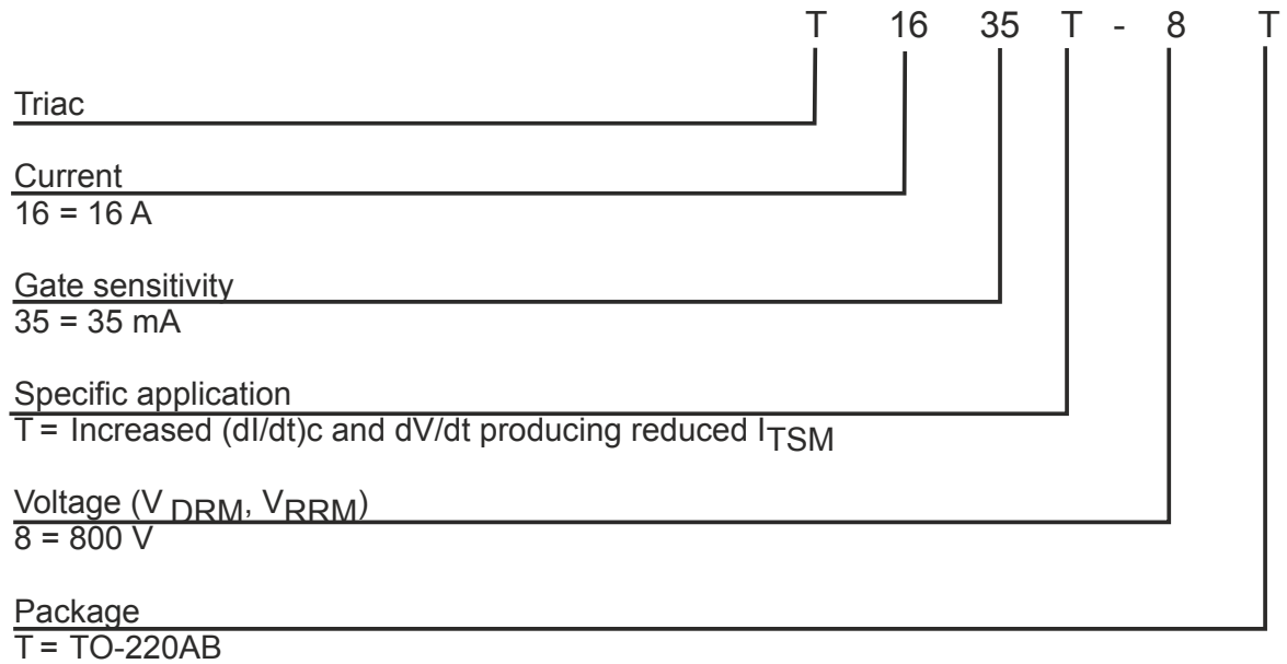
Figure 15. Ordering information scheme
