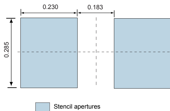
Figure 12. Stencil opening recommendations
