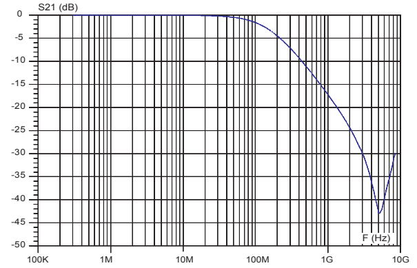
Figure 7. S21 attenuation
