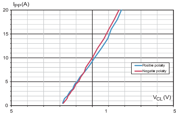
Figure 6. TLP
