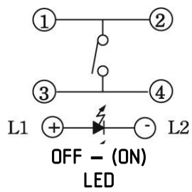
Circuitry
