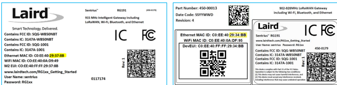
Figure 4: Bottom label (Standard GW – Left, AS923 & AU915 Region Supported/Latest Version – Right)– last three bytes of the Ethernet MAC address highlighted
