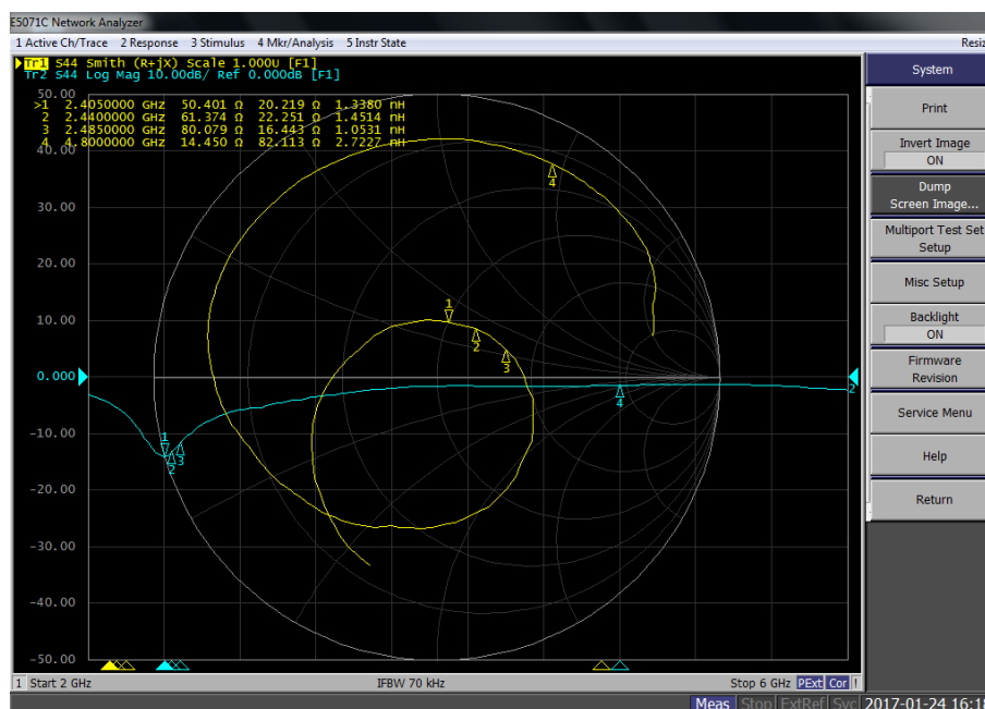
Figure 4.2. Impedance and Reflection of the Inverted-F Antenna of the BRD4161A Board Measured from the Matching Output
