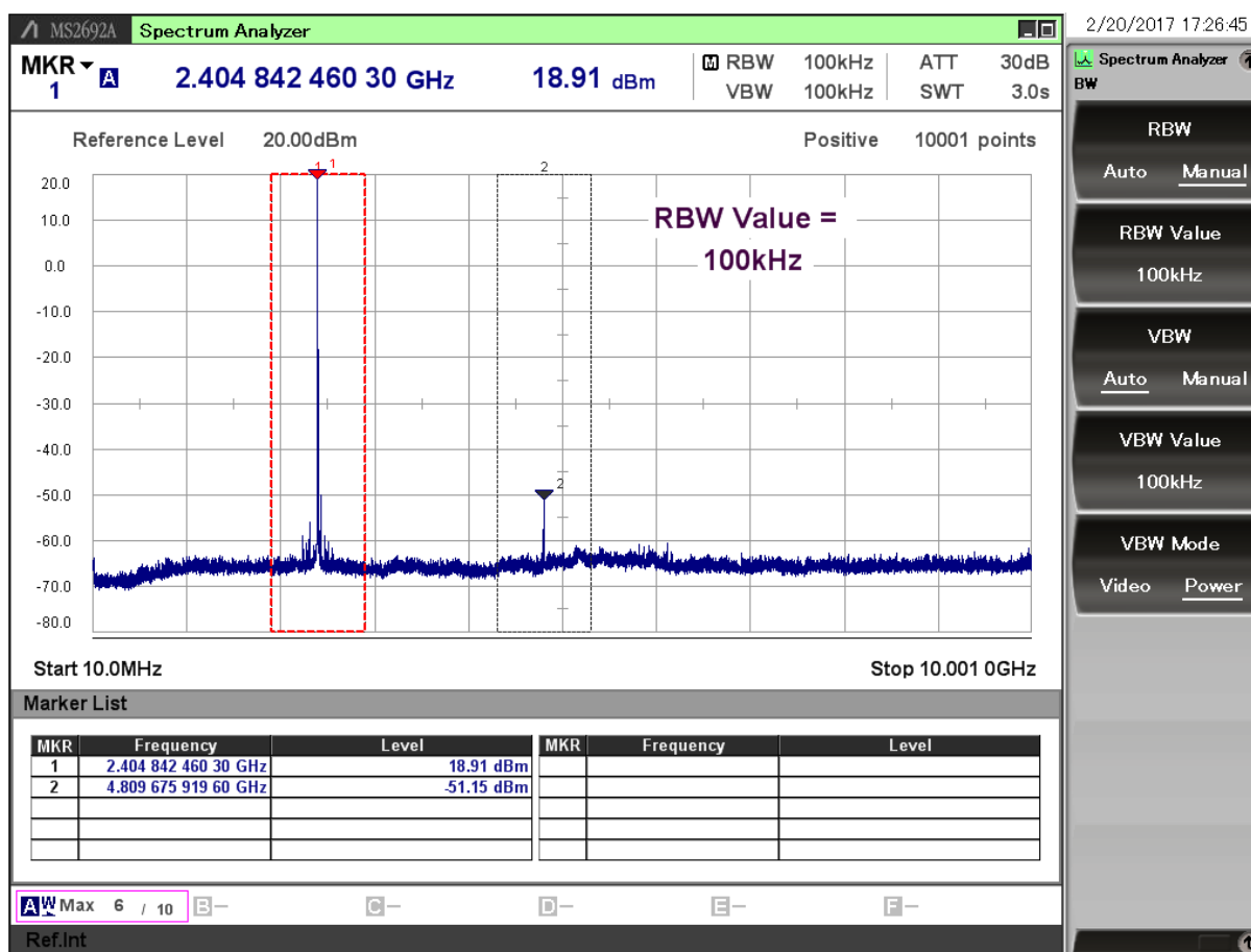
Figure 7.1. Typical Output Spectrum of the BRD4161A
