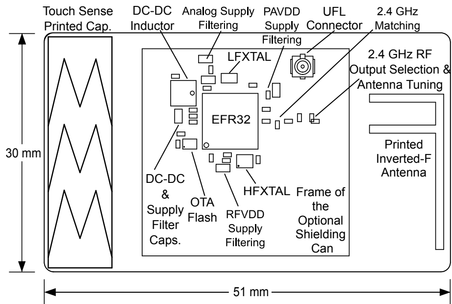
Figure 5.1. BRD4161A Top View
