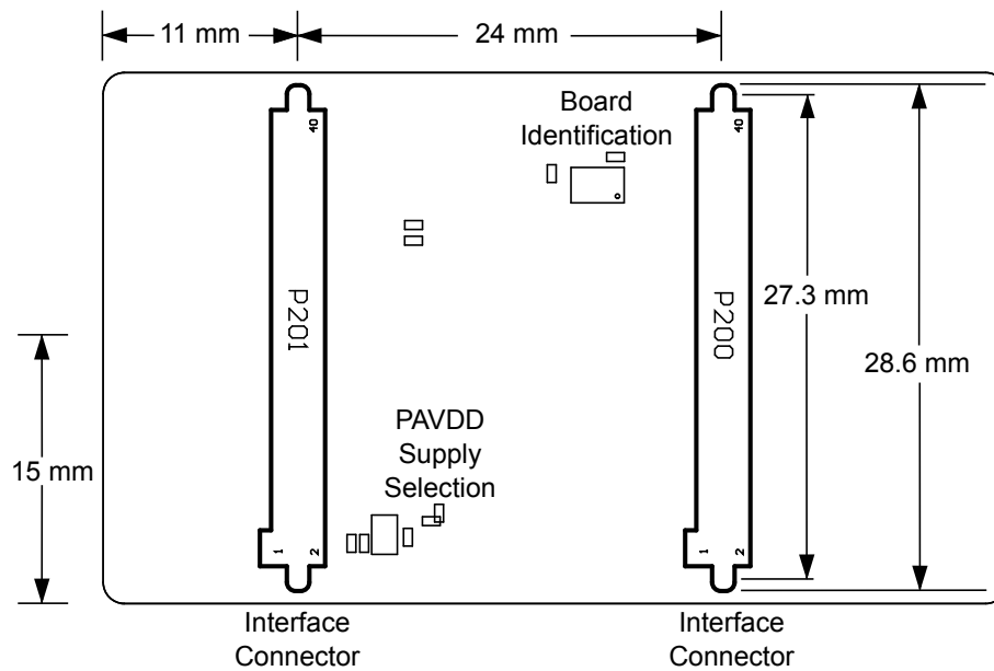
Figure 5.2. BRD4161A Bottom View
