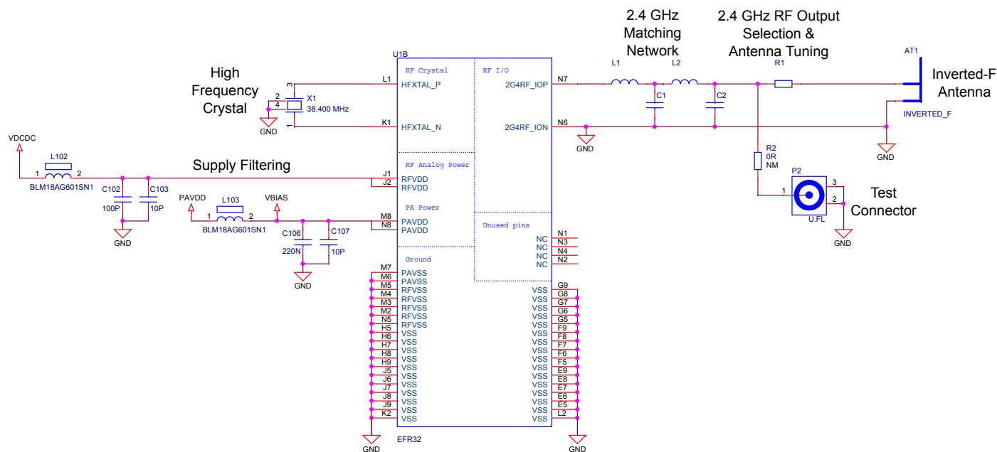
Figure 4.1. Schematic of the RF Section of the BRD4161A
