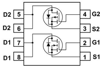
SOP-8 top view
