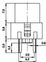
Mounting
