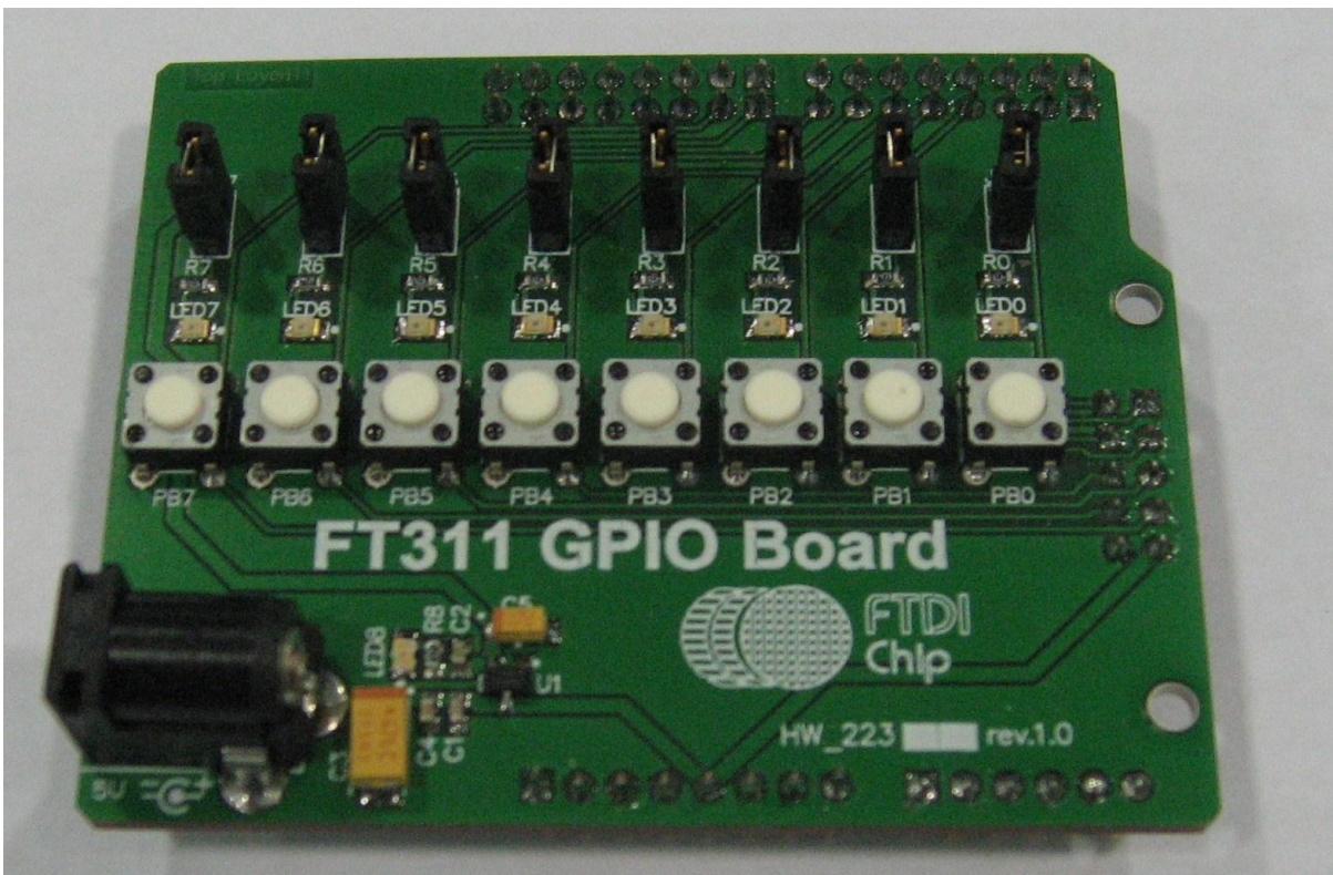
Figure 1.1 : FT311 GPIO Board
