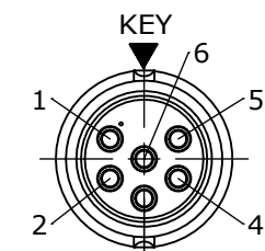
WIRING END W6280-6PG-P-3XX
