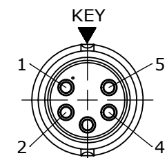
WIRING END W6280-5PG-P-3XX
