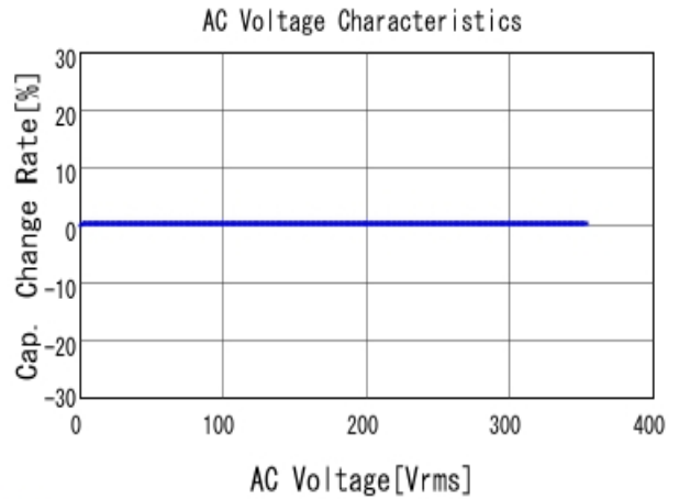
■ GRM31B7U3A391JW31 C-AC Voltage capchange, DCOV, 25.0d
