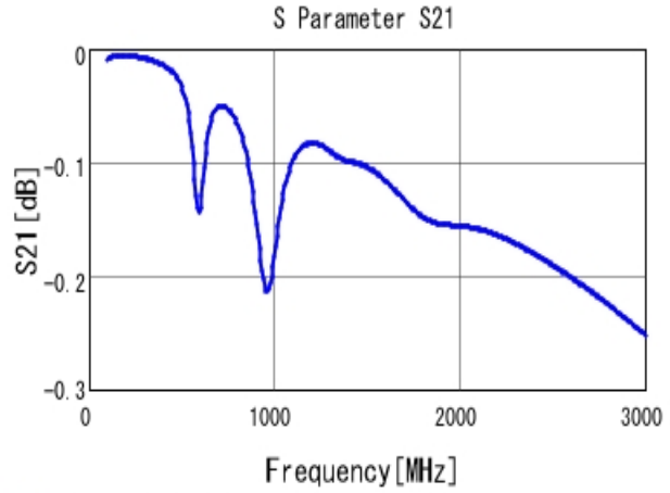
■ GRM31B7U3A391JW31 S21 DCOV, 25degC
