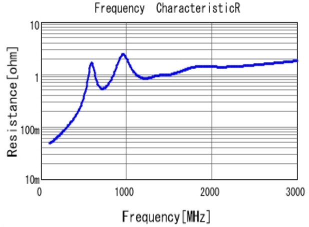
■ GRM31B7U3A391JW31 R DCOV, 25degC
