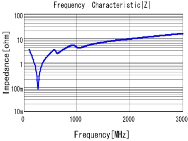
■ GRM31B7U3A391JW31 |Z| DCOV, 25degC
