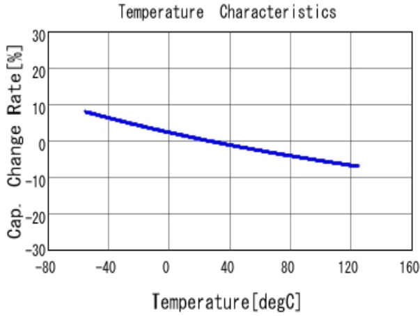
■ GRM31B7U3A391JW31 C-Temp. capchange, DCOV, AC1Vrms
