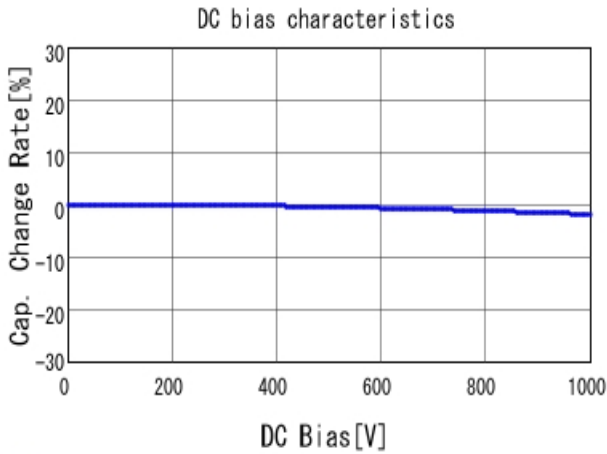
■ GRM31B7U3A391JW31 C-DC bias capchange, 25.0degC, AC1V
