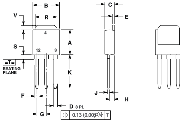
DPAK-3 Case 369D
