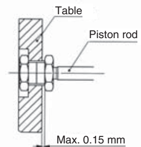
Connecting part of piston rod and table
