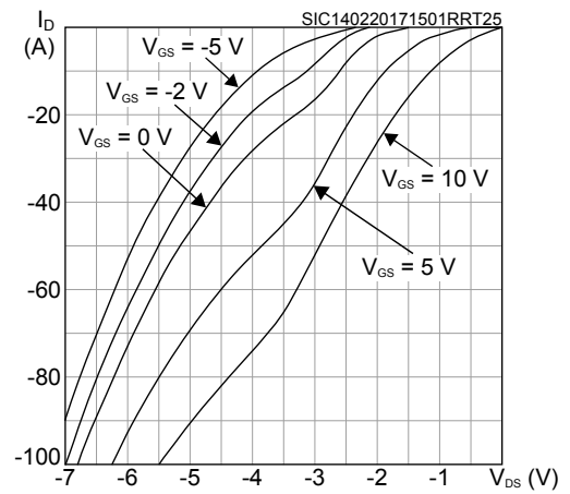
Figure 14. Reverse conduction characteristics ( T_J = 25\text{ }^\circ\text{C} )
