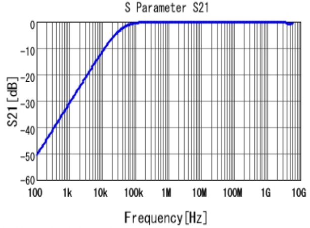
■ GCM21BR71H473KA37 S21 DCOV, 25degC
