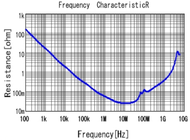
GCM21BR71H473KA37 R DCOV, 25degC
