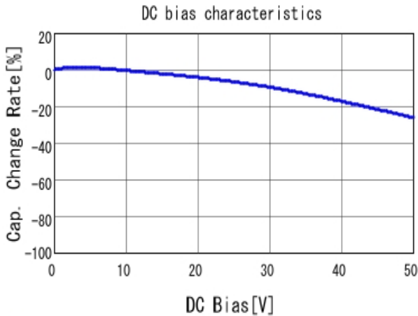
GCM21BR71H473KA37 C-DC bias capchange, 25.0degC, AC1.
