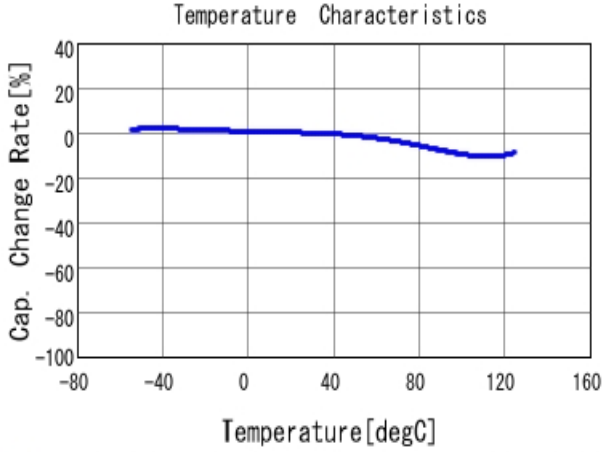
■ GCM21BR71H473KA37 C-Temp. capchange, DCO. 0V, AC1.0Vrm
