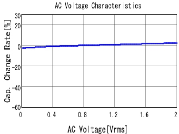
GCM21BR71H473KA37 C-AC Voltage capchange, DCOV, 25.0d
