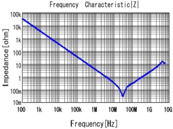
GCM21BR71H473KA37 |Z| DCOV, 25degC
