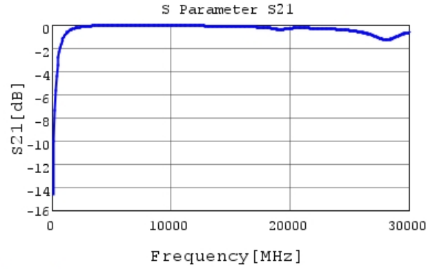
GRM0225C1E3R0WA03 S21 DCOV, 25degC
