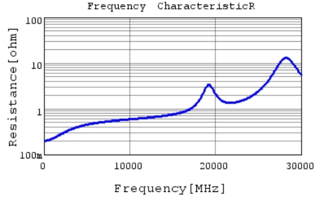
GRM0225C1E3R0WA03 R DCOV, 25degC
