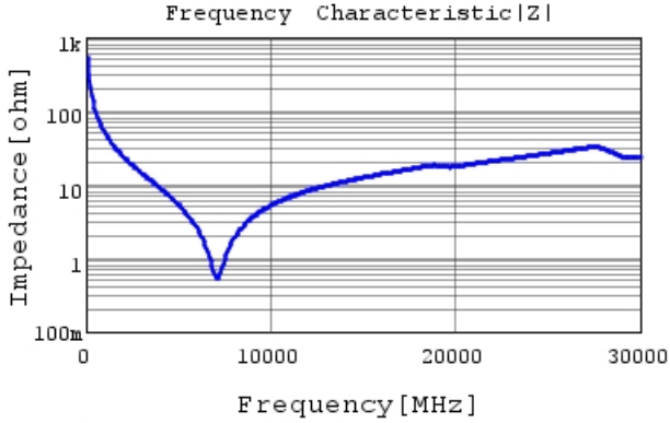
GRM0225C1E3R0WA03 |Z| DCOV, 25degC
