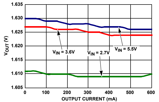
FIGURE 4. LOAD REGULATION
