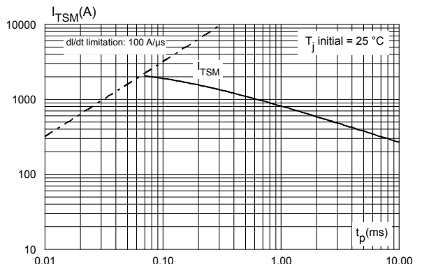
Figure 10. Non repetitive surge peak on-state current for a sinusoidal pulse with width t_p < 10\text{ ms}
