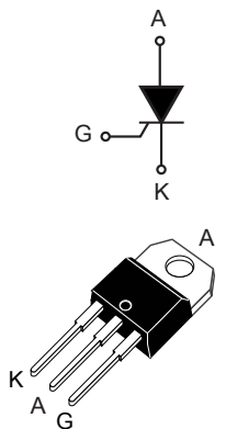
TO-220AB
