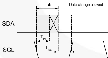
Figure 5. Data Transfer Timing
