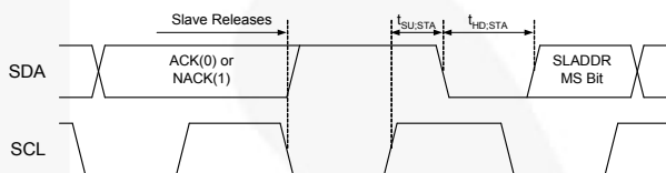
Figure 8. Repeated STOP Timing
