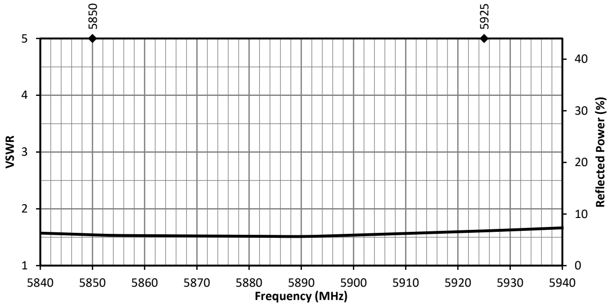
Figure 3. ANT-V2X-IPW1-NP Antenna VSWR, Free Space
