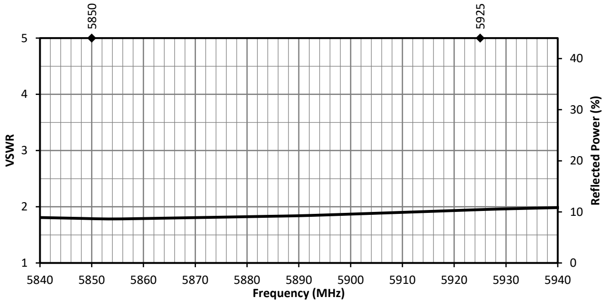
Figure 11. ANT-V2X-IPW1-NP Antenna VSWR, Center of Ground Plane
