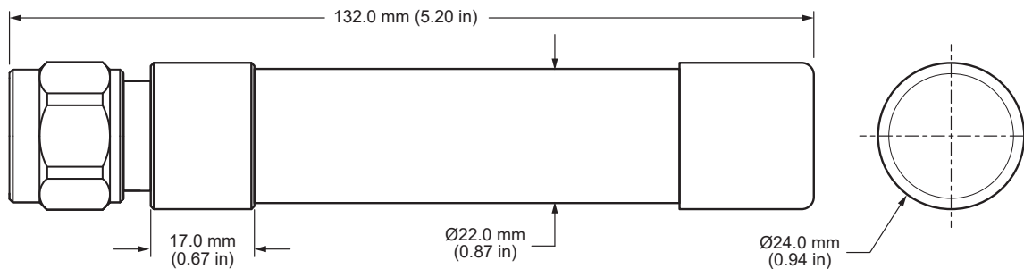
Figure 1. ANT-5GW-IPW2-NP Antenna Dimensions
