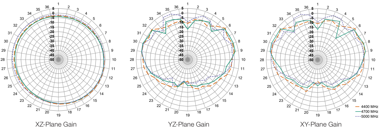
Figure 16. Radiation Patterns for ANT-5GW-IPW2-NP, Center of Ground Plane
