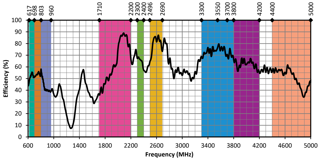
Figure 8. ANT-5GW-IPW2-NP Antenna Efficiency, Free Space
