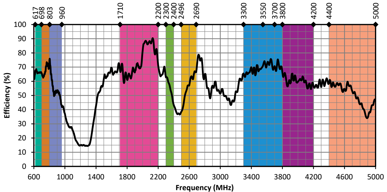
Figure 15. ANT-5GW-IPW2-NP Antenna Efficiency, Center of Ground Plane
