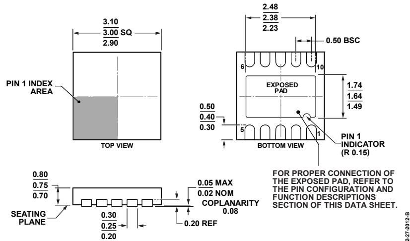
Figure 32. 10-Lead Lead Frame Chip Scale Package [LFCSP_WD] 3 mm x 3 mm Body, Very Very Thin, Dual Lead (CP-10-9) Dimensions shown in millimeters
