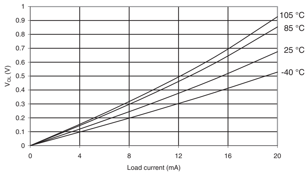
Figure 31-56. I/O Pin Output Voltage vs. Sink Current ( V_{CC} = 3V )
