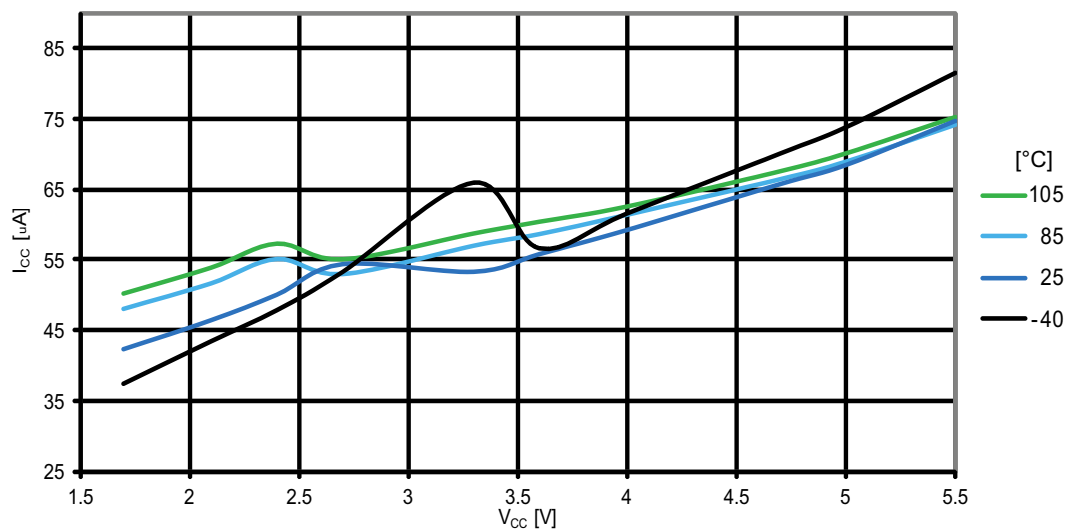
Figure 31-157. Atmel ATmega1284P: Analog comparator current vs. V_{CC} .
