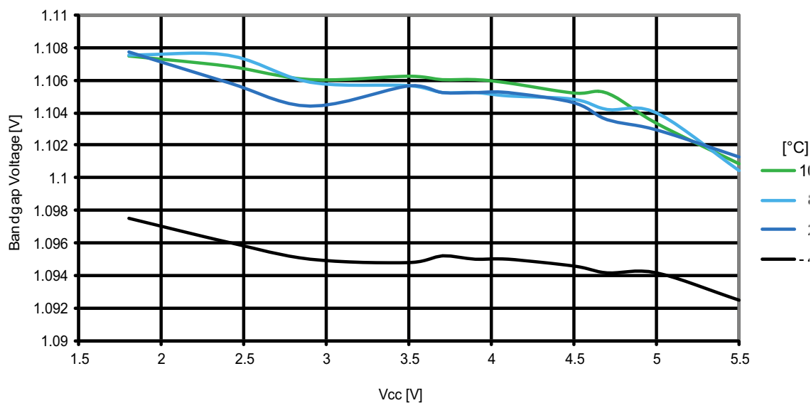
Figure 31-28. Atmel ATmega164PA: Calibrated bandgap voltage vs. V_{CC} .
