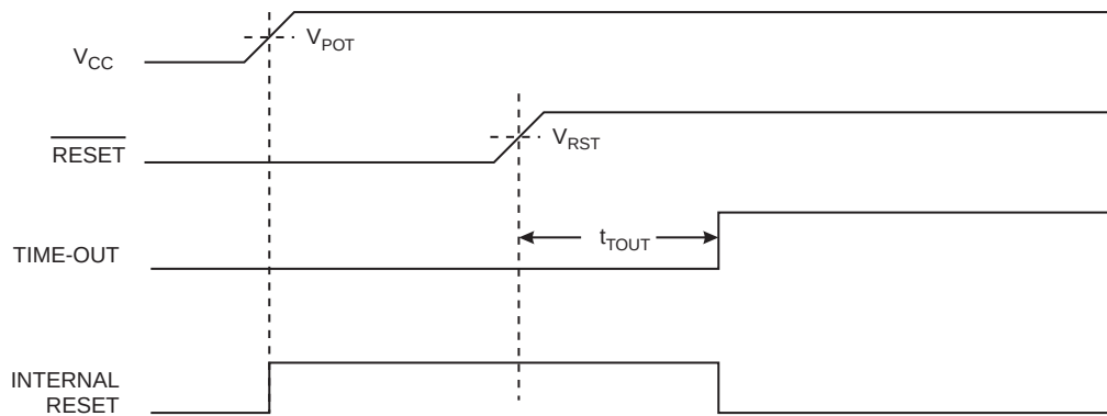
Figure 11-3. MCU Start-up, RESET Extended Externally.
