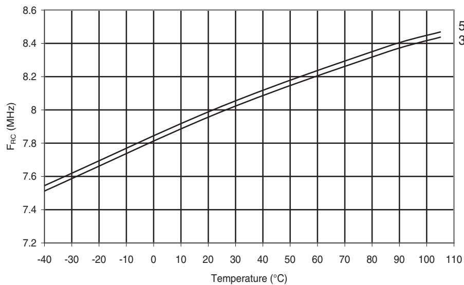
Figure 31-72. Calibrated 8 MHz RC Oscillator vs. Temperature
