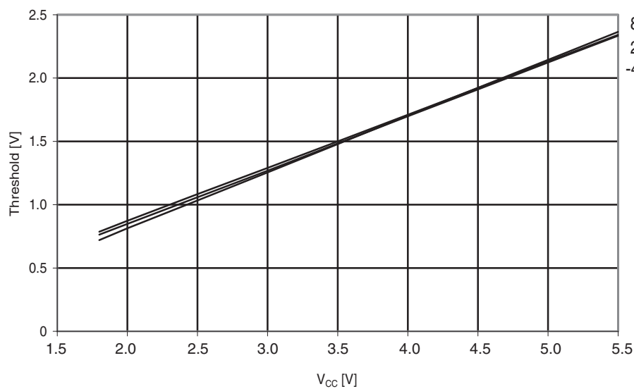
Figure 30-271. Atmel ATmega644PA: I/O pin input threshold vs. V_{CC} ( V_{IL} , I/O pin read as '0').
