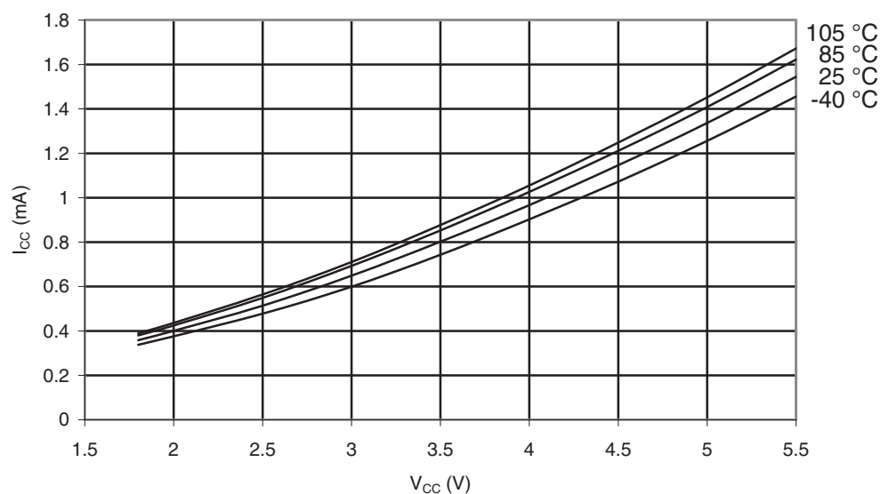
Figure 31-45. Idle Supply Current vs. V_{CC} (Internal RC Oscillator, 8 MHz)
