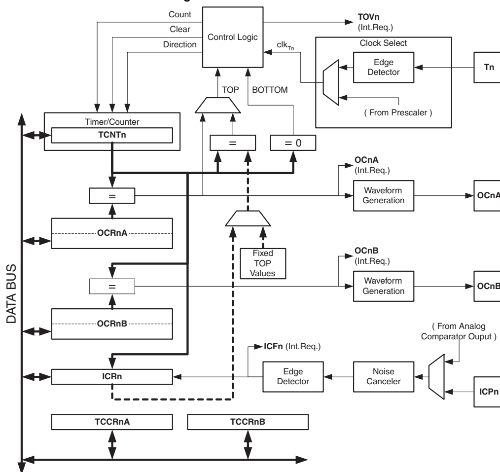
Figure 16-1. 16-bit Timer/Counter block diagram (Note:).
