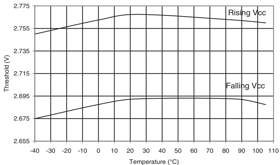
Figure 31-106. BOD Threshold vs. Temperature ( V_{CC} = 2.7V )
