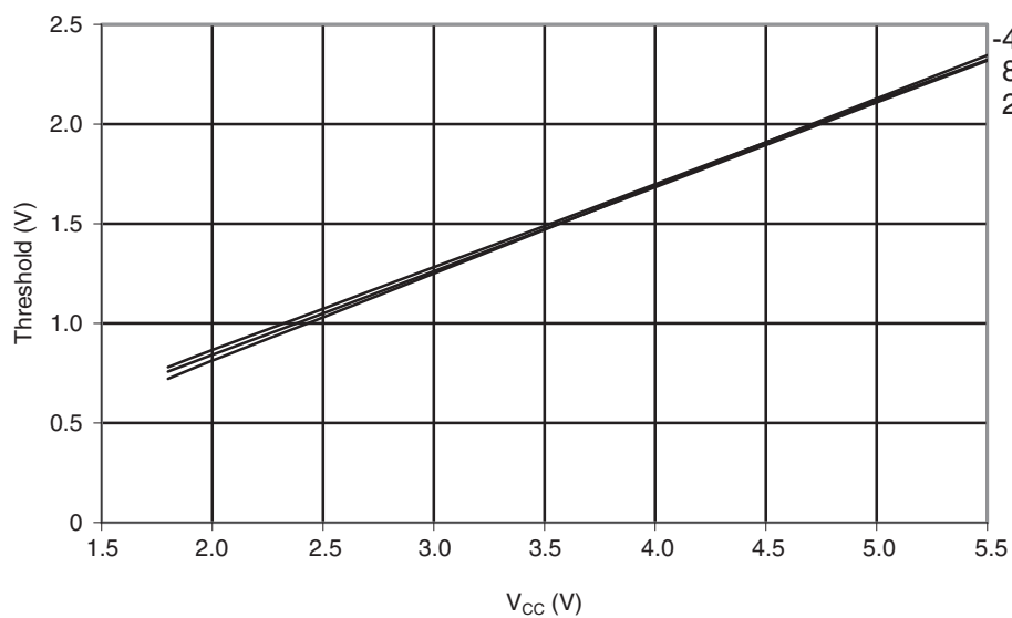
Figure 30-374. Atmel ATmega1284P: Reset pin input threshold vs. V_{CC} ( V_{IL} , I/O pin read as '0').
