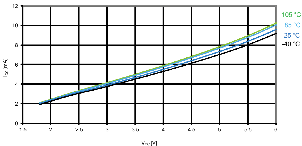
Figure 31-120. Atmel ATmega1284P: Active supply current vs. V CC (internal RC oscillator, 8MHz)
