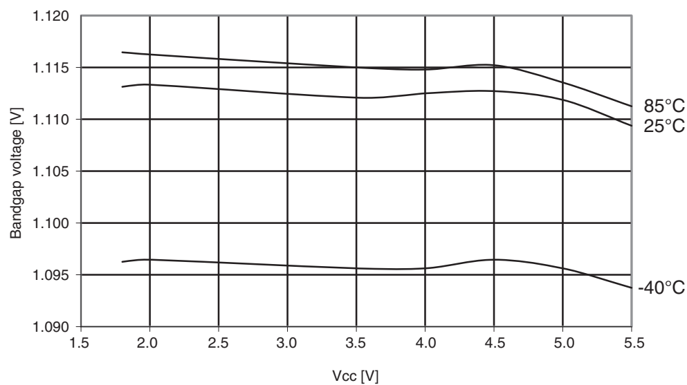
Figure 30-329. Atmel ATmega1284: Calibrated bandgap voltage vs. V_{CC} .
