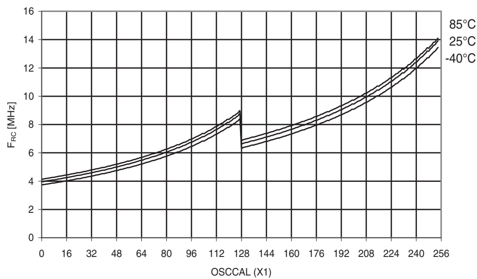
Figure 30-187. Atmel ATmega324PA: Calibrated 8MHz RC oscillator vs. OSCAL value.
