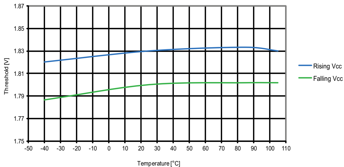
Figure 31-148. Atmel ATmega1284P: BOD threshold vs. temperature ( V_{BOT} = 1.8V ).
