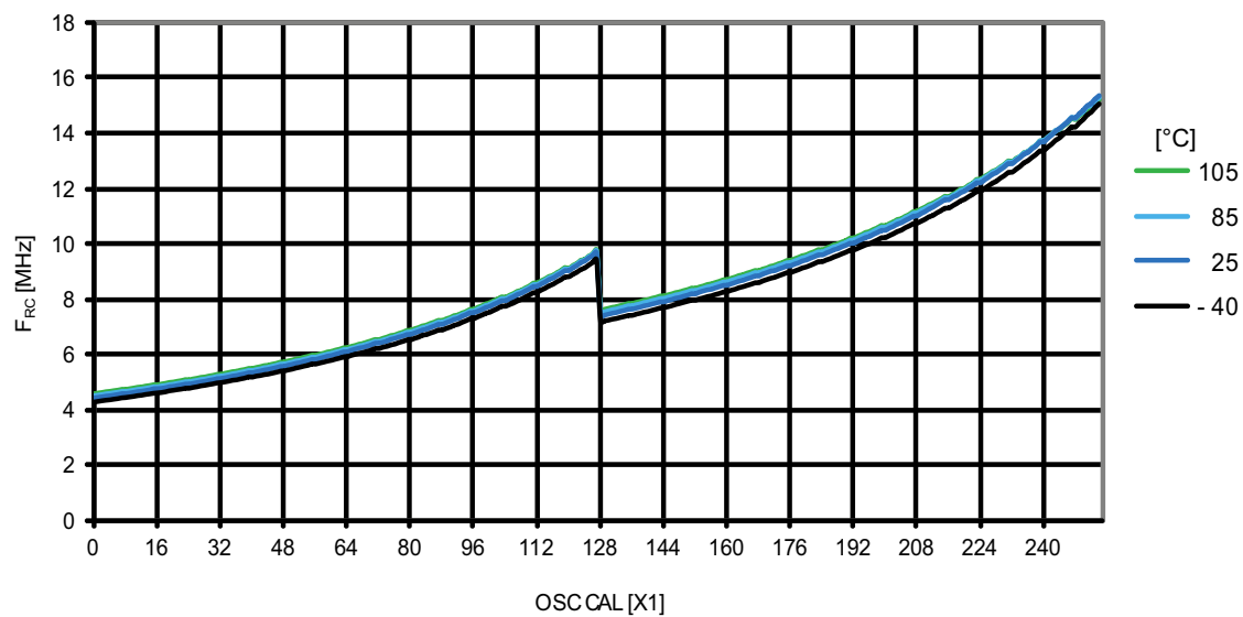
Figure 31-34. Atmel ATmega164PA: Calibrated 8MHz RC oscillator vs. OSCAL value.
