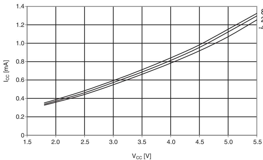
Figure 30-249. Atmel ATmega644PA: Active supply current vs. V_{CC} (internal RC oscillator, 1MHz).
