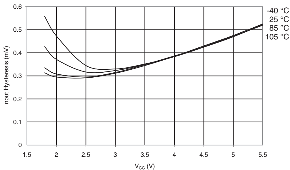
Figure 31-101. I/O Pin Input Hysteresis vs. V_{CC}
