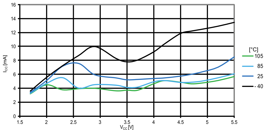
Figure 31-160. Atmel ATmega1284P: Programming current vs. V_{CC} .
