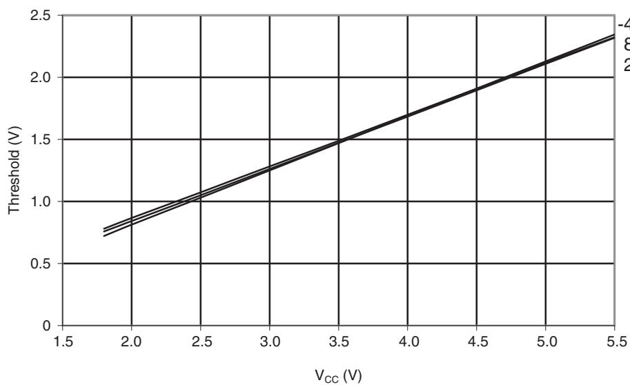
Figure 30-324. Atmel ATmega1284: Reset pin input threshold vs. V_{CC} ( V_{IL} , I/O pin read as '0').
