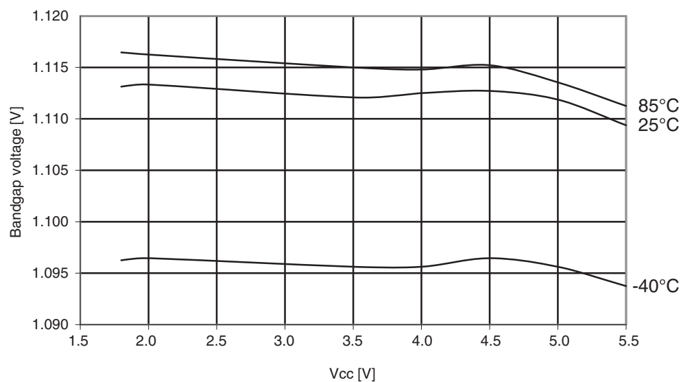
Figure 30-379. Atmel ATmega1284P: Calibrated bandgap voltage vs. V_{CC} .
