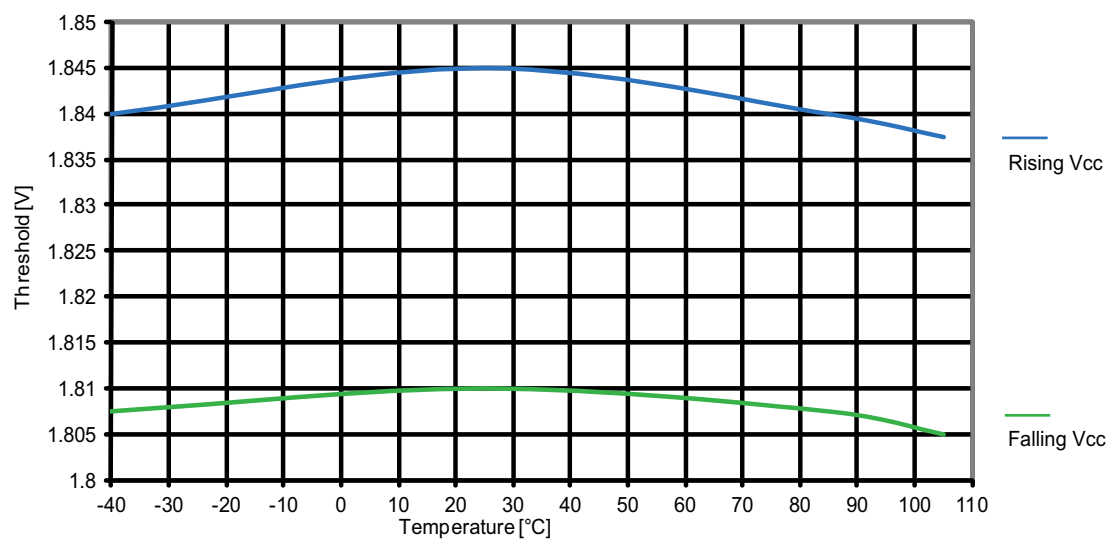
Figure 31-27. Atmel ATmega164PA: BOD threshold vs. temperature ( V_{BOT} = 1.8V ).
