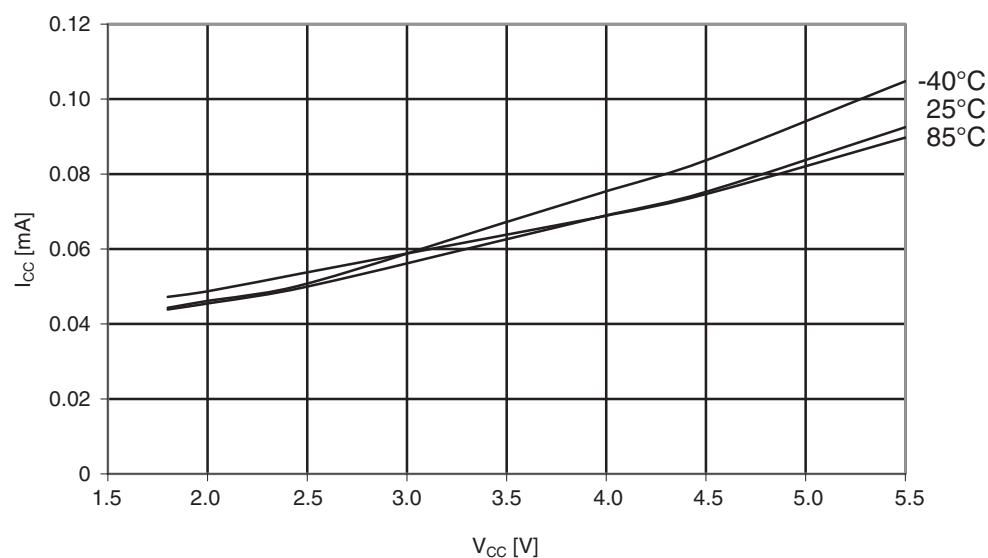
Figure 30-206. Atmel ATmega644A: Idle supply current vs. V_{CC} (internal RC oscillator, 128kHz).
