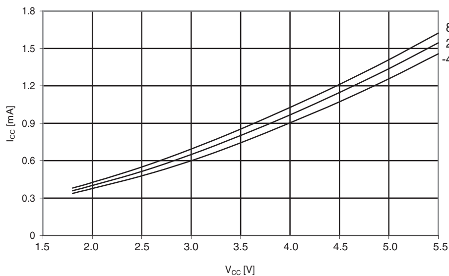
Figure 30-106. Atmel ATmega324A: Idle supply current vs. V_{CC} (internal RC oscillator, 8MHz).
