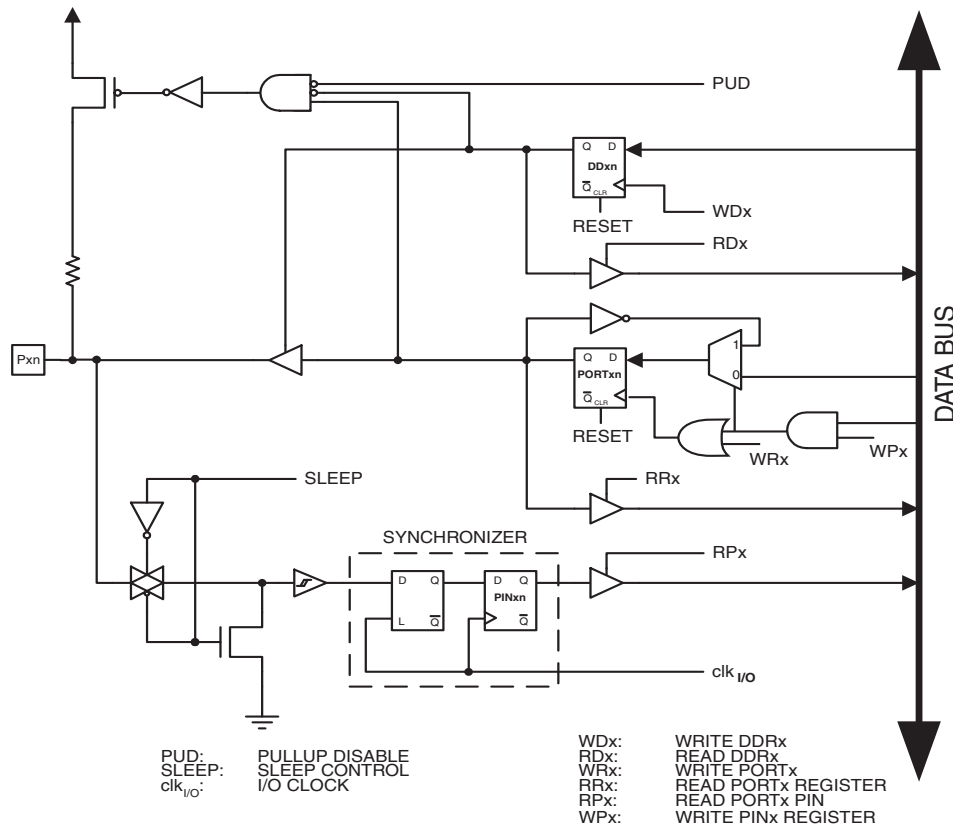
Figure 14-2. General digital I/O (1) .
