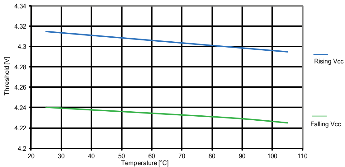
Figure 31-25. Atmel ATmega164PA: BOD threshold vs. temperature ( V_{BOT} = 4.3V ).
