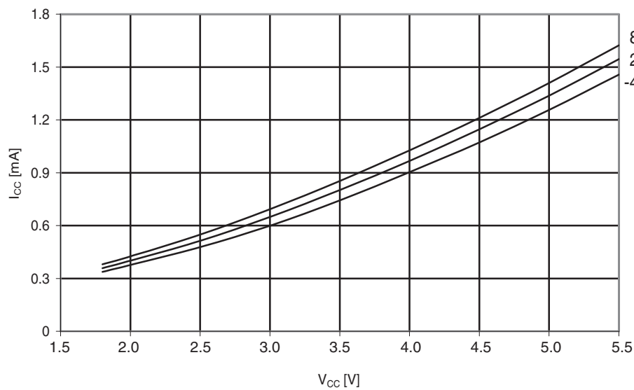
Figure 30-155. Atmel ATmega324PA: Idle supply current vs. V_{CC} (internal RC oscillator, 8MHz).
