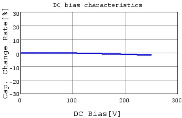
GRM31B7U2E103JW31 C-DC bias capchange, 25.0c
