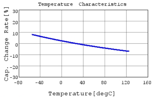
GRM31B7U2E103JW31 C-Temp. capchange, DCOV, 1
