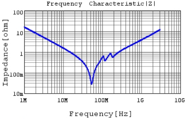
GRM31B7U2E103JW31 |Z| DCOV, 25degC
