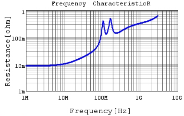
GRM31B7U2E103JW31 R DCOV, 25degC
