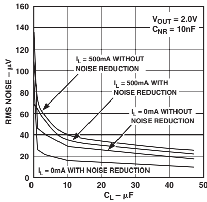
TPC 17. RMS Noise vs. C_L (10 Hz to 100 kHz)
