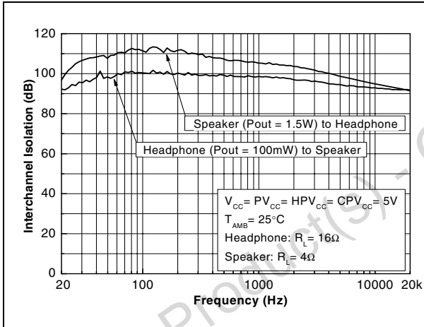
Figure 34. Inter-channel isolation vs. frequency
