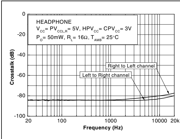
Figure 32. Crosstalk vs. frequency
