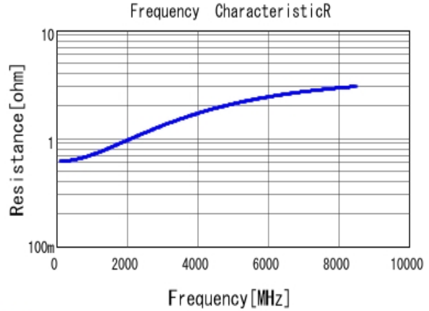
■ GRM1885C1HR50BA01 R DC0V, 25degC
