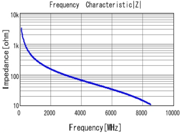
■ GRM1885C1HR50BA01 |Z| DC0V, 25degC
