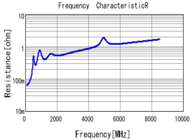
GCM1885C1H681JA16 R DC0V, 25degC
