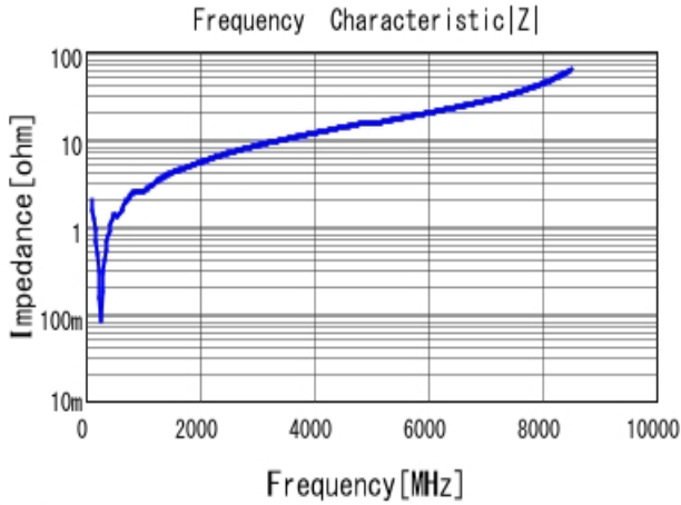
GCM1885C1H681JA16 |Z| DC0V, 25degC
