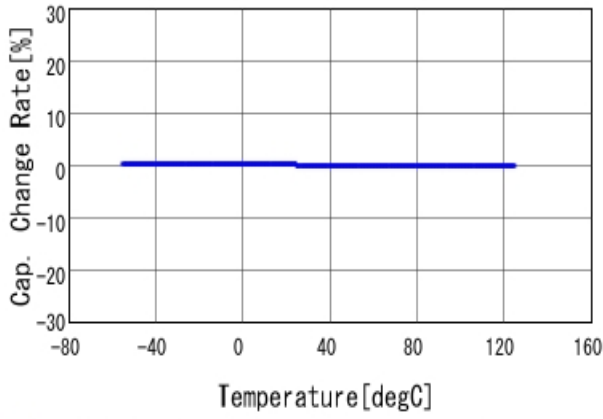
Temperature Characteristics
