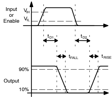
Figure 9. Inverting
