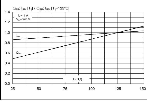
Figure 9: Relative variation of dynamic parameters versus junction temperature
