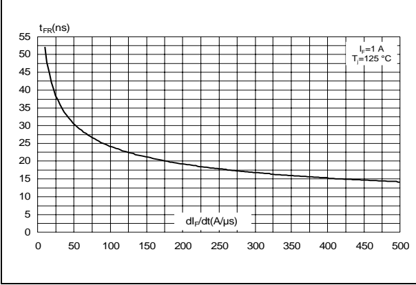
Figure 11: Forward recovery time versus di_F / dt (typical values)
