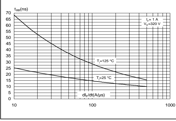
Figure 7: Reverse recovery time versus di_F / dt (typical values)
