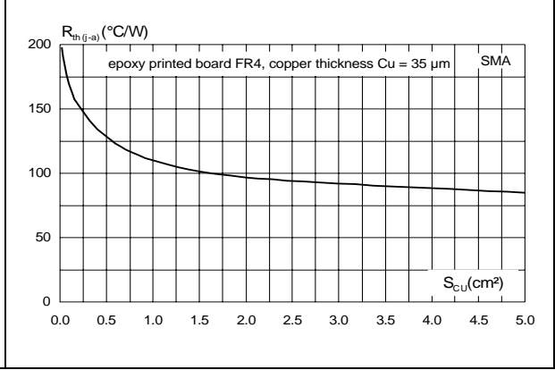
Figure 12: Thermal resistance junction to ambient total versus copper surface under each lead (SMA)
