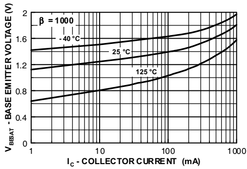
Figure 3. Base-Emmitter Saturation Voltage vs. Collector Current
