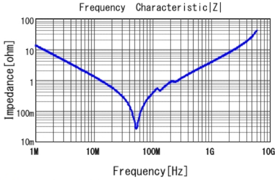
■ GRM3195C1H123JA01 |Z| DCOV, 25degC
