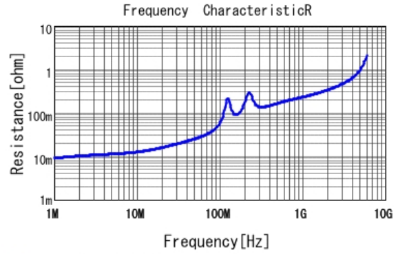
■ GRM3195C1H123JA01 R DCOV, 25degC
