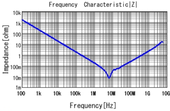
■ GRM21BR71A105KA01 |Z| DCOV, 25degC
