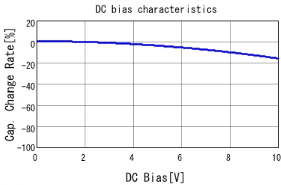
■ GRM21BR71A105KA01 C-DC bias capchange, 25.0degC, AC1.
