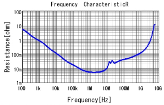
■ GRM21BR71A105KA01 R DCOV, 25degC
