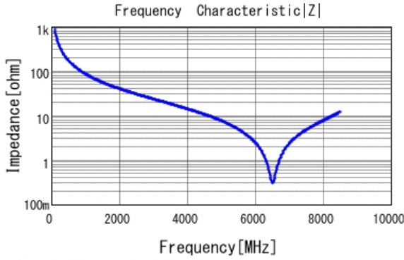
■ GJM1555C1H1R8WB01 |Z| DCOV, 25degC
