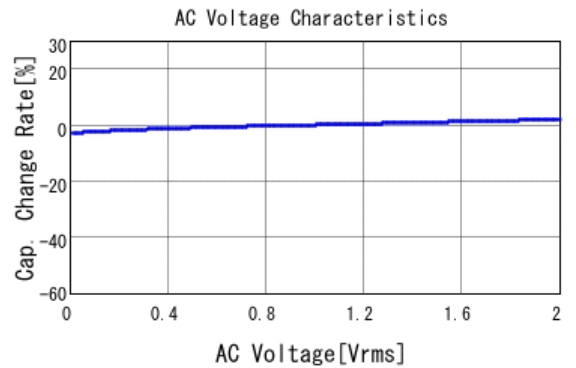
GCM155R72A102KA37 C-AC Voltage capchange, DC0V, 25.0d
