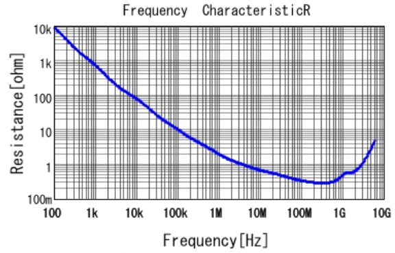
GCM155R72A102KA37 R DC0V, 25degC
