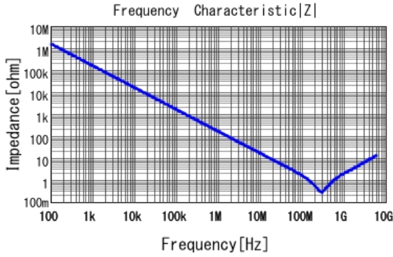
GCM155R72A102KA37 |Z| DC0V, 25degC
