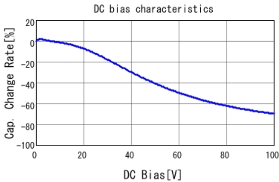
GCM155R72A102KA37 C-DC bias capchange, 25.0degC, AC1.
