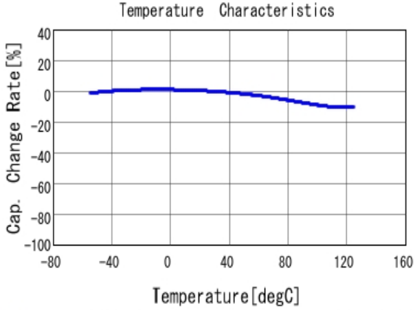
GCM31MR71H105KA55 C-Temp. capchange, DC0.0V, AC1.0V r m
