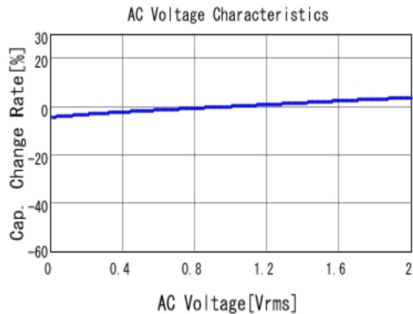
GCM31MR71H105KA55 C-AC Voltage capchange, DC0V, 25.0d
