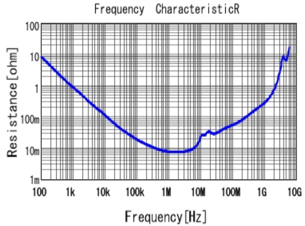
GCM31MR71H105KA55 R DC0V, 25degC
