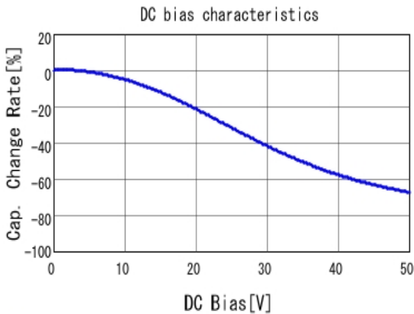
GCM31MR71H105KA55 C-DC bias capchange, 25.0degC, AC1.
