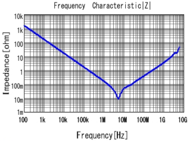
GCM31MR71H105KA55 |Z| DC0V, 25degC
