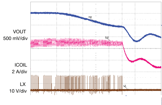
Fig. 18 - Over Current Protection, I_{VALLEY} = 4 \text{ A} , Time = 20 \mu\text{s}/\text{div}
