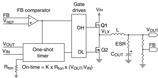
Fig. 24 - On-Time Generation
