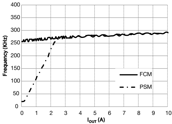
Fig. 9 - Switching Frequency - PSM vs. FCM ( V_{DD} = 5\text{ V} , V_{OUT} = 1.5\text{ V} , V_{IN} = 12\text{ V} )
