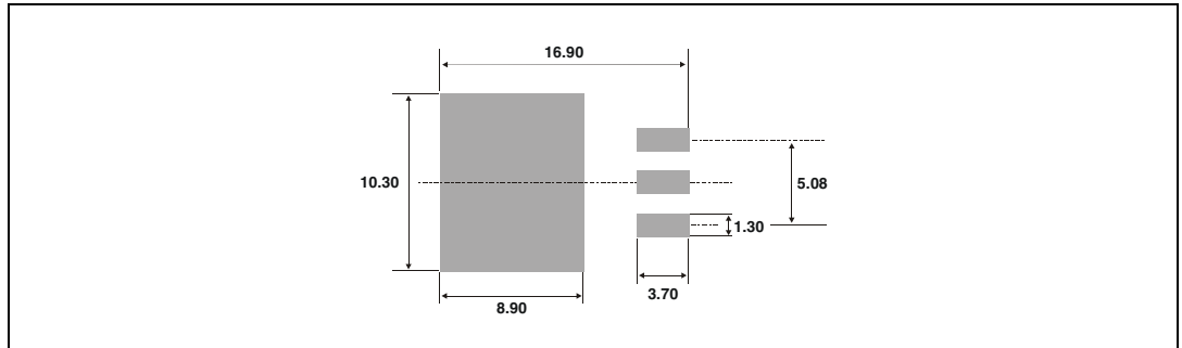
Figure 14. Footprint (dimensions in mm)
