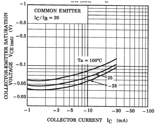
Fig. 10.22 RN2404 V_{CE(sat)}-I_C
