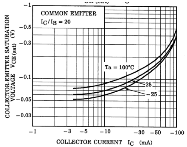
Fig. 10.20 RN2402 V_{CE(sat)}-I_C
