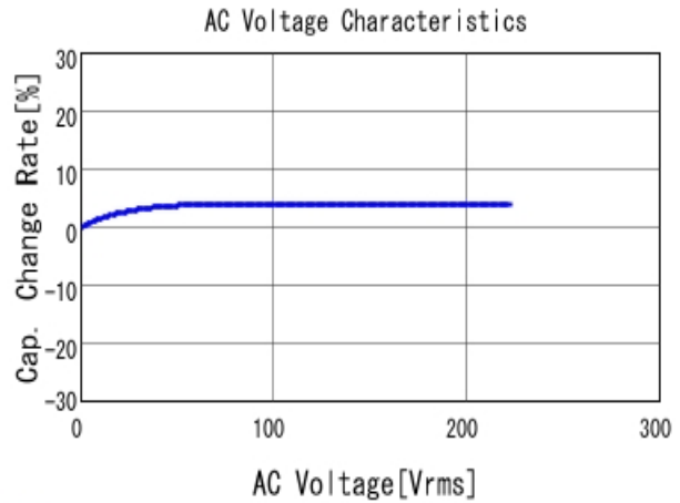
■ GRM31A7U2J151JW31 C-AC Voltage capchange, DCOV, 25.0d
