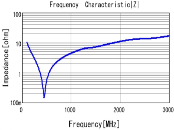
■ GRM31A7U2J151JW31 |Z| DCOV, 25degC
