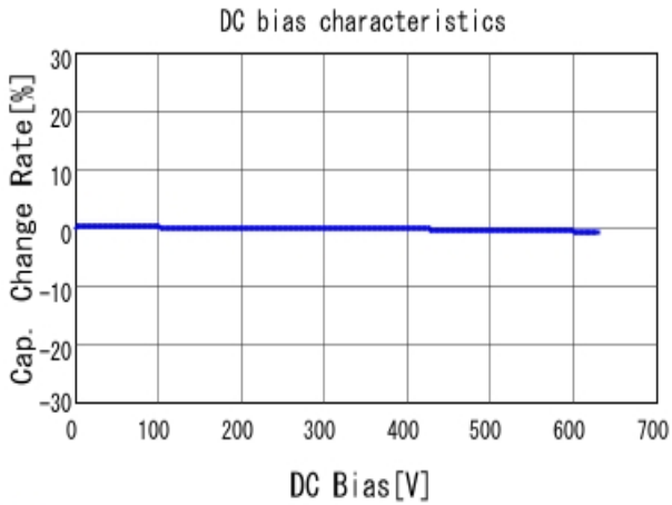
■ GRM31A7U2J151JW31 C-DC bias capchange, 25.0degC, AC1V
