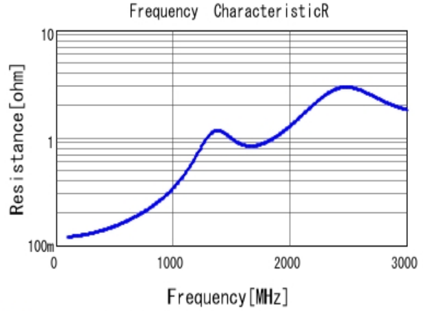
■ GRM31A7U2J151JW31 R DCOV, 25degC
