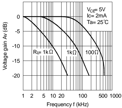
Fig.11 Frequency Response
