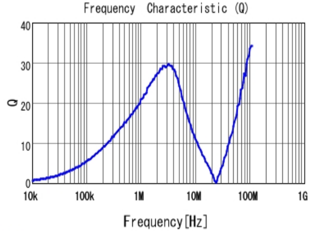
■ LQH2MCN680K02 Q
