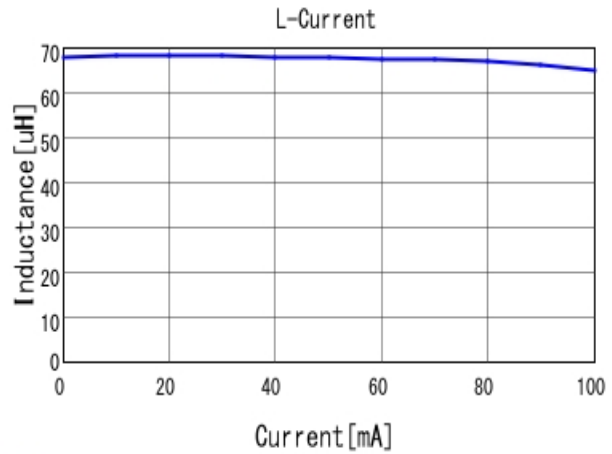
■ LQH2MCN680K02 L-Current 20degC
