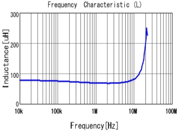
■ LQH2MCN680K02 L
