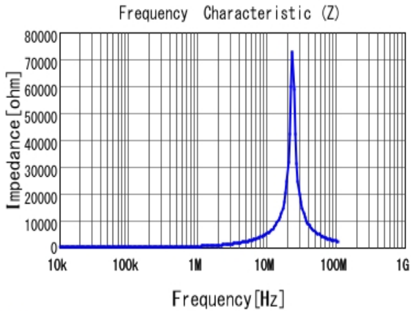
■ LQH2MCN680K02 |Z|
