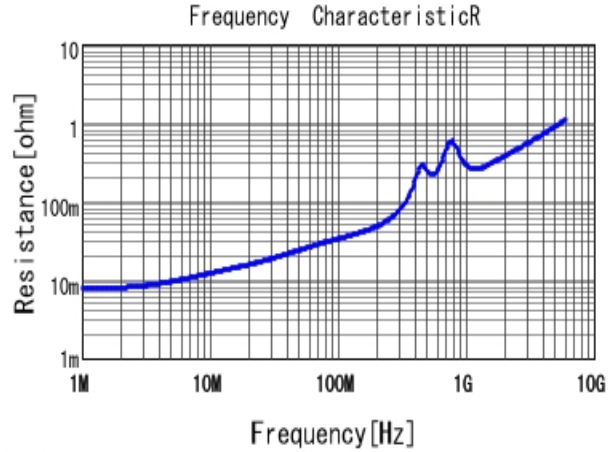
■ GRM2165C1H182JA01 R DCOV, 25degC
