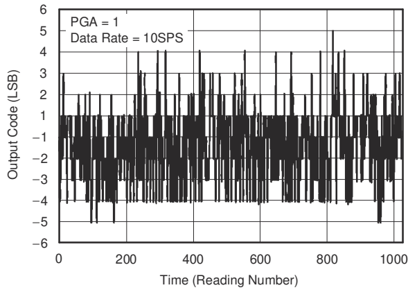
Figure 6-1. Noise Plot
