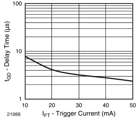
Fig. 9 - Trigger Current vs. Delay Time
