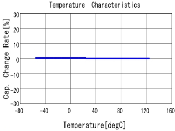
■ GCM1885C2A120JA16 C-Temp. capchange, DCOV, AC1Vrms
