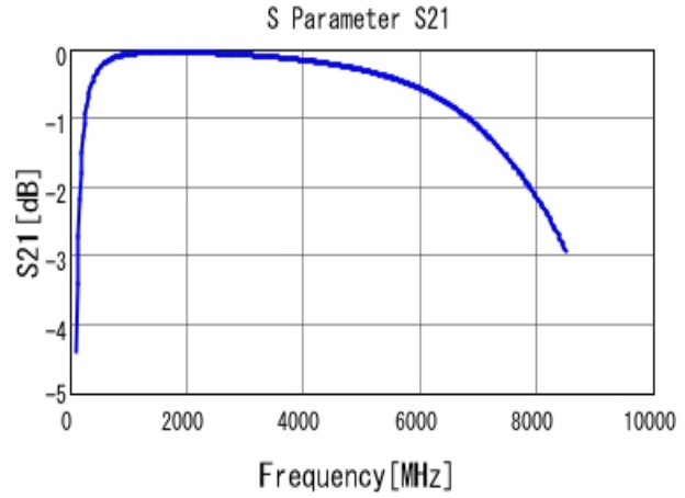
■ GCM1885C2A120JA16 S21 DCOV, 25degC
