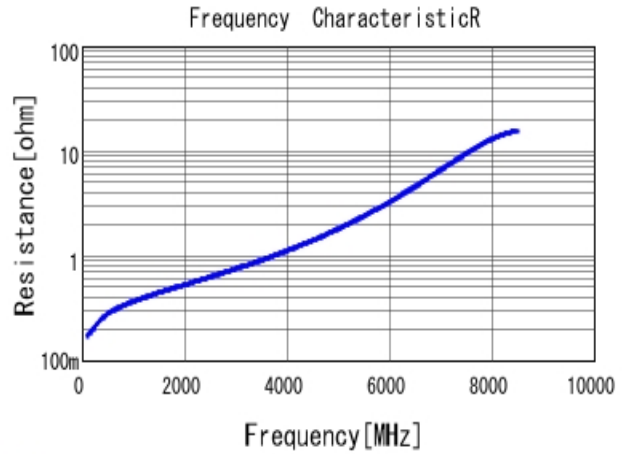
GCM1885C2A120JA16 R DC0V, 25degC
