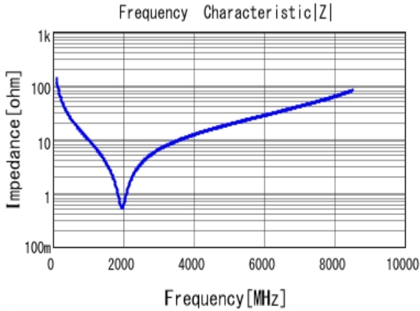
GCM1885C2A120JA16 |Z| DC0V, 25degC
