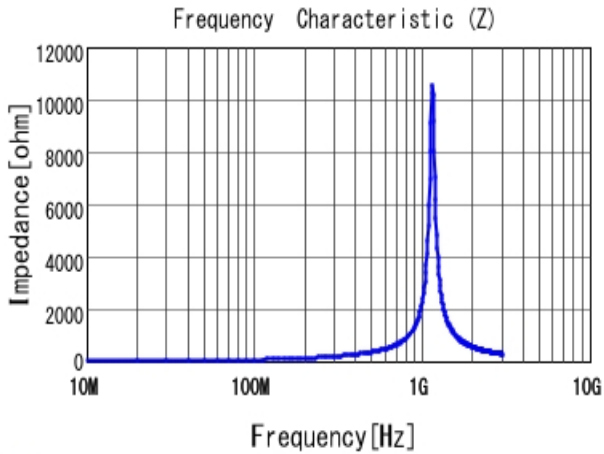
■ LQP03TNR10J02 |Z|
