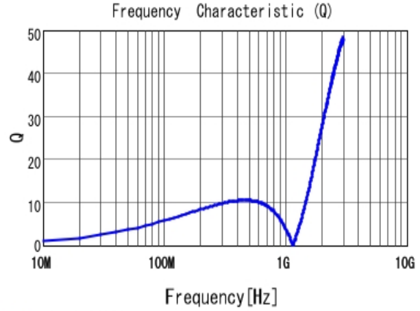
■ LQP03TNR10J02 Q
