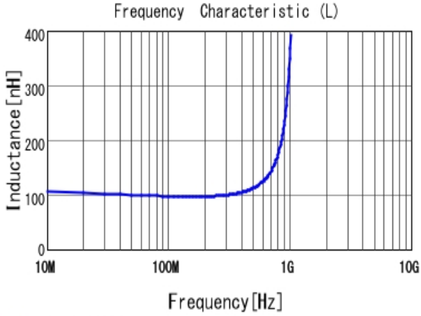
■ LQP03TNR10J02 L
