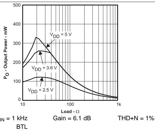
Figure 29. Output Power vs Load
